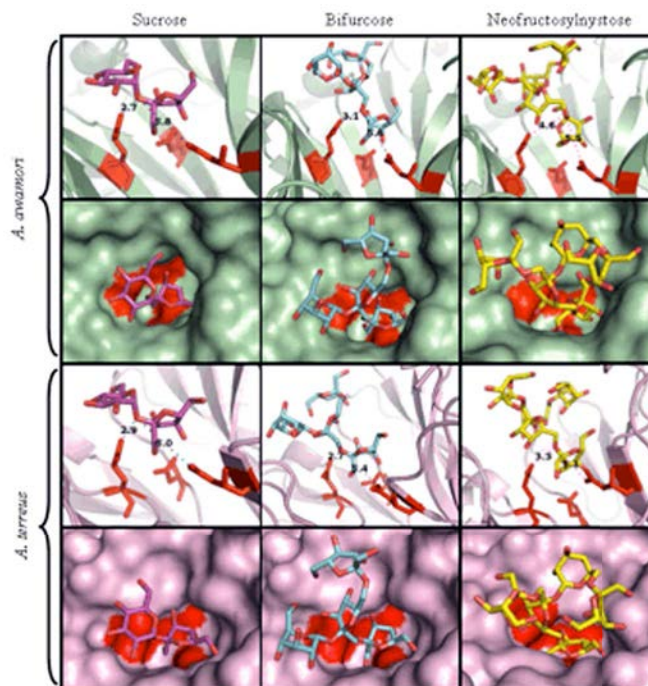
Figure 2. AAEI and ATPF dockings with sucrose (pink), Bifurcose (blue) and Neofructosylmystose (yellow) as substrates. Distance in Å from the catalytic residues and the glycosidic bond are shown in black numbers.
