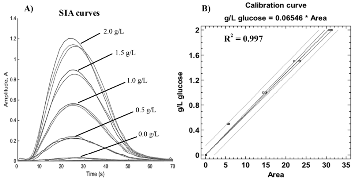
Figure 1. A) Response curves obtained from the processed samples in the SIA system and the calibration curve. B) linear regression with areas of the calibration curve.
