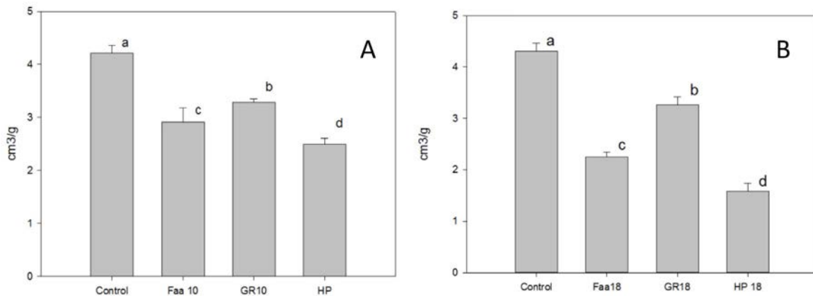
Figure 2. Specific volume of baked bread. A: (10% fructans), B: (18% fructans). Faa: agave fructans (Olifrufructine®), GR: Chicory fructans GR, HP: Chicory fructans HP.
